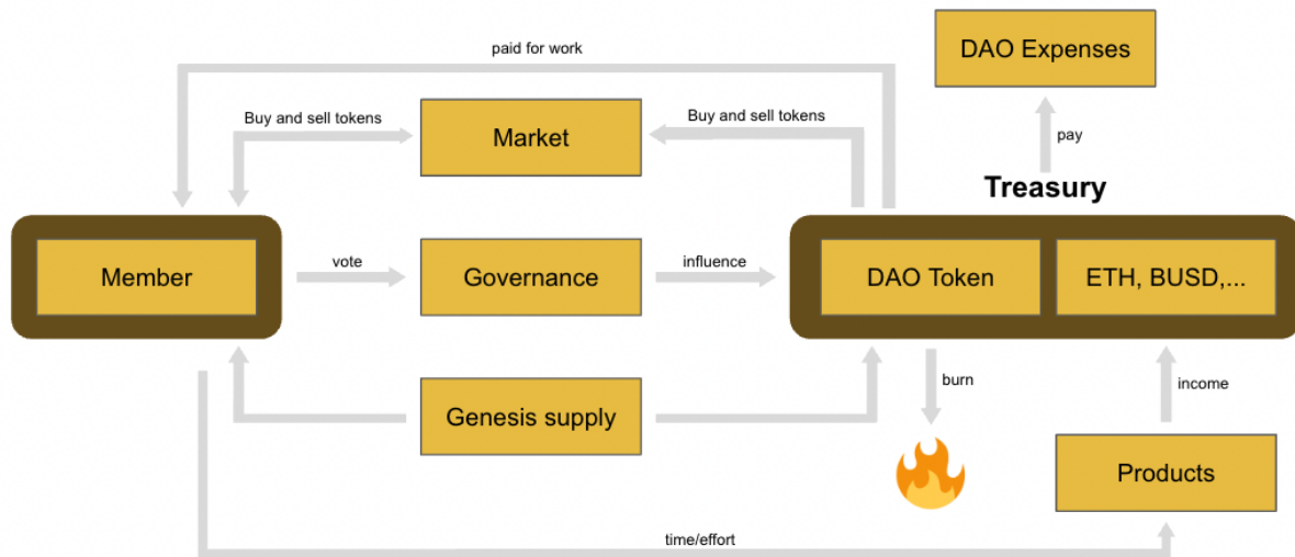
Figure 3: DAO Operational Design - Members and Treasury are two crucial components of DAOs. Tokens are an essential building block to connect these two.
